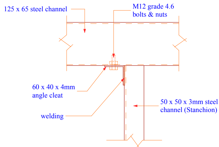
BEAM CONNECTION DETAIL FOR ST 5
