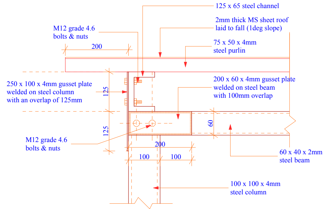
DETAIL FOR JOINT B
