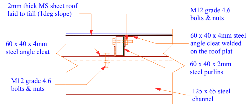
DETAIL FOR JOINT B
