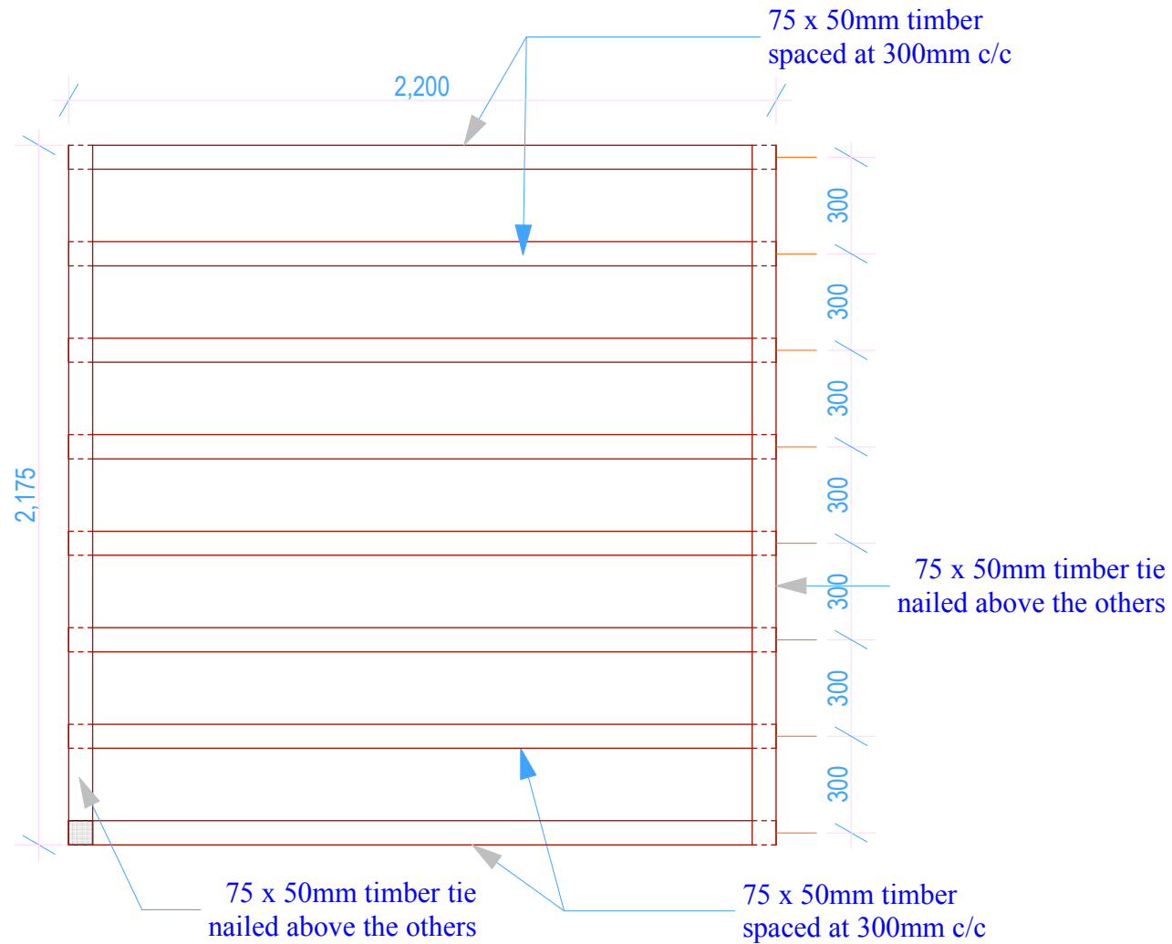
TIMBER PLATFORM
