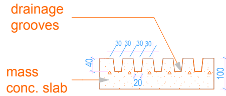
DRAINAGE GROOVES (DETAIL F)
