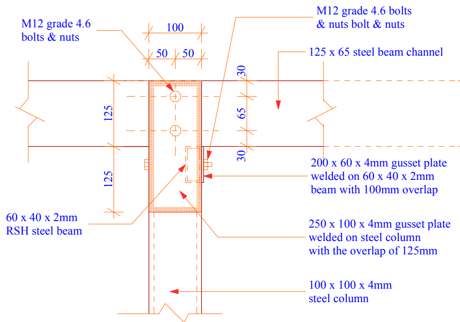
DETAIL FOR JOINT A
