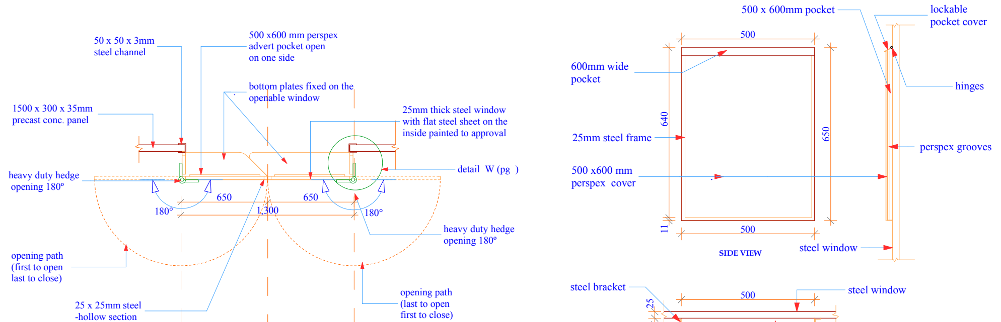
PLAN
