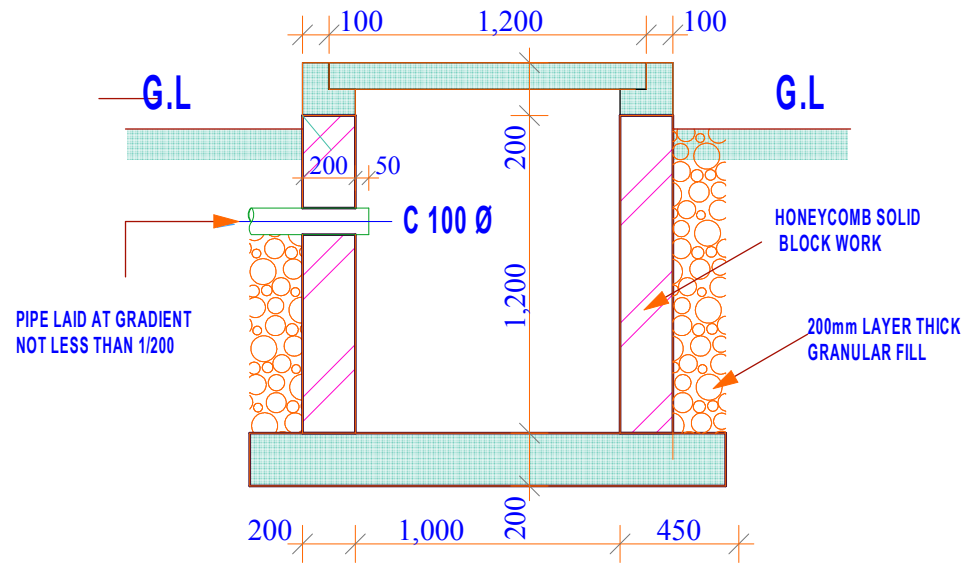
LONGITUDINAL SECTION THROUGH SECTION G-G
