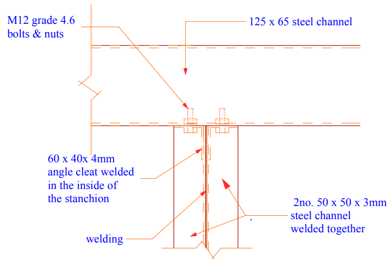
BASE DETAIL FOR ST 4
